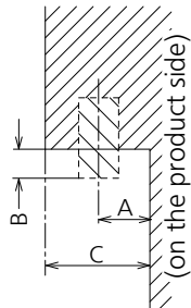
Sectional view of terminal a (MICRO SD / SERIAL IN / LAN / USB TYPE-C / USB TYPE-A / USB TYPE-A)
