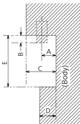
Sectional view of terminal a (HDMI 2 / HDMI 3 / LAN / SERIAL IN)
